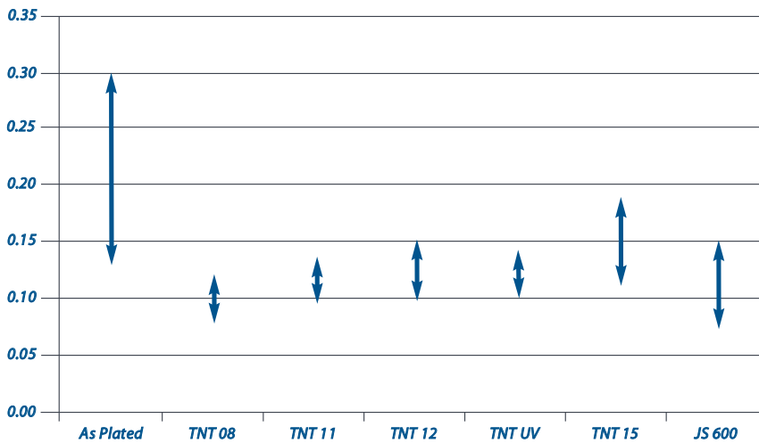
CoF - MacDermid Friction Control Fluids on Zinc Electroplate
